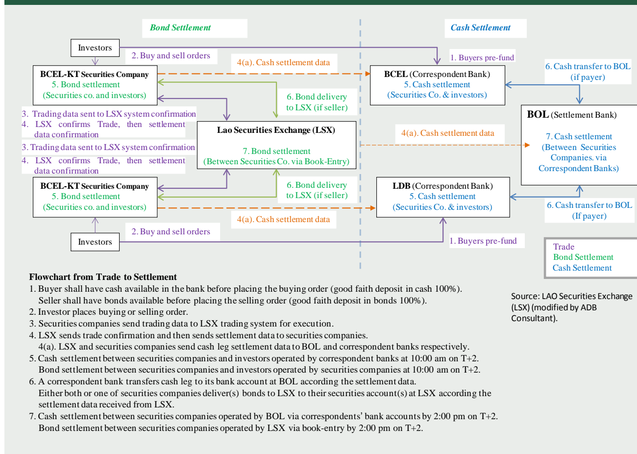
Figure LA02: Flowchart of Listed Corporate Bond Settlement
